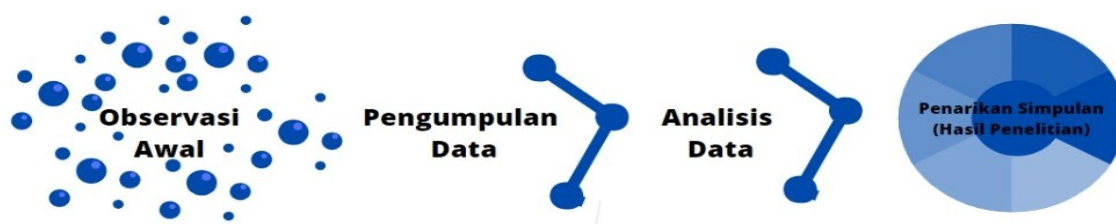
Gambar 1. Alur Penelitian
